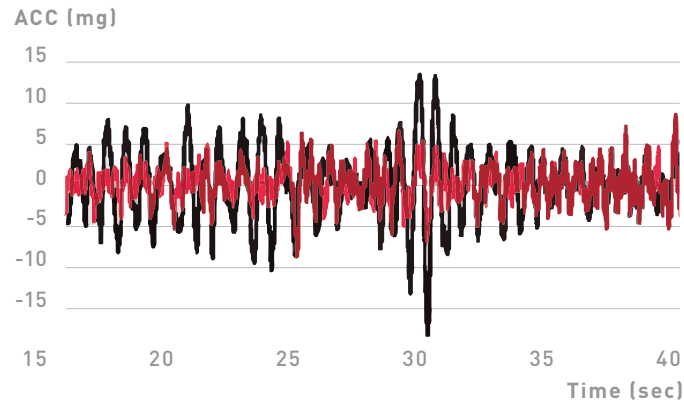
Figure 1 ● Standard Fujitec Roller ● Fujitec ARG
